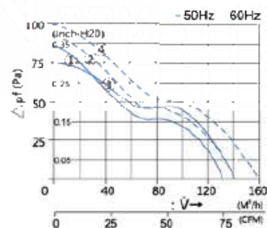
Performance FK 9923....
