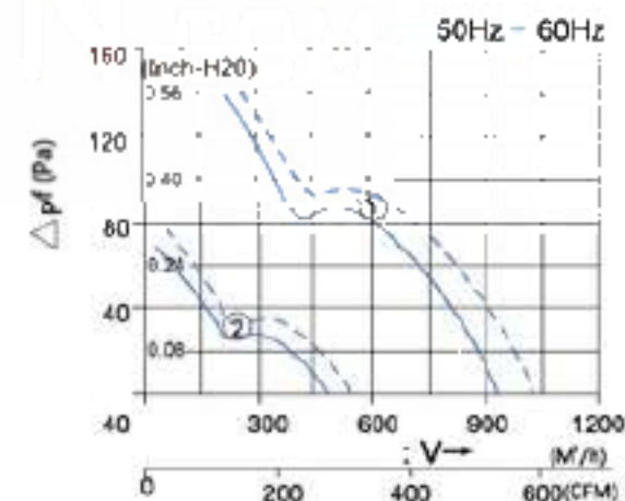
Performance FK 9926....
