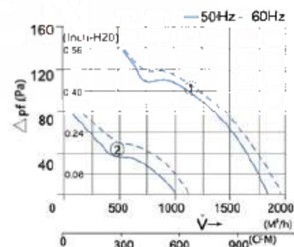
Drawing FK 9926....
