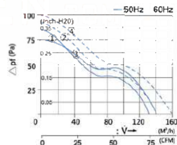
Performance FK 9922....
