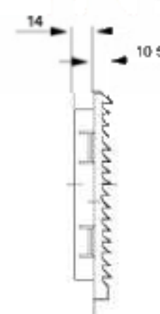
Exit filter FKL 6622.300
