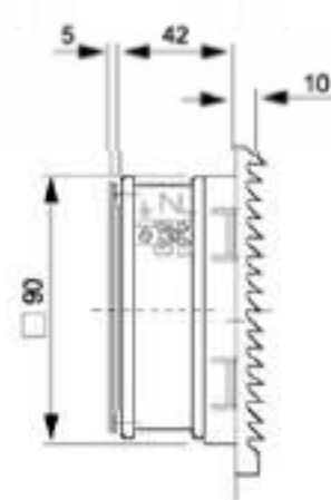
Fans and filters FKL 6621.230
