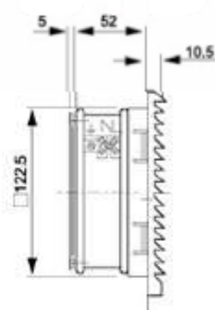
Fans and filters FKL 6622.230
