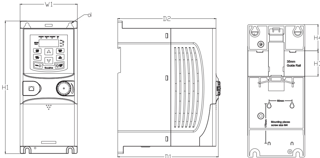
Rail mounting
