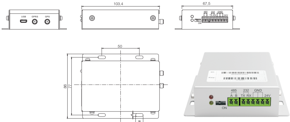
GPRS module installation dimensions
