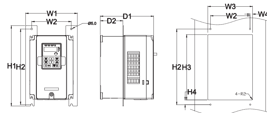
Flange installation
