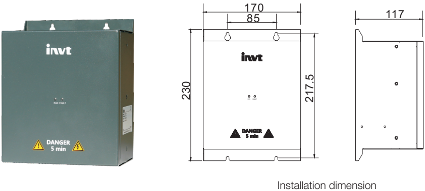
Installation dimension
